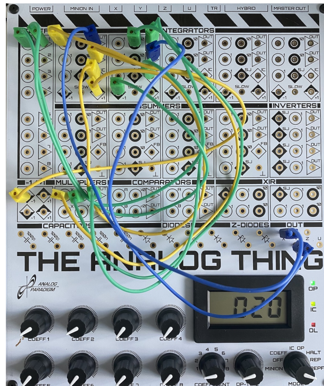
Figure 3: Setup of THE ANALOG THING for generating a Gaussian function
