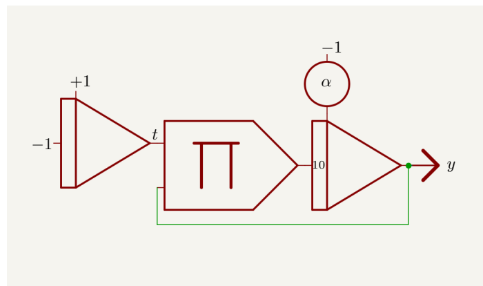
Figure 1: Analog computer setup for generating a Gaussian function
