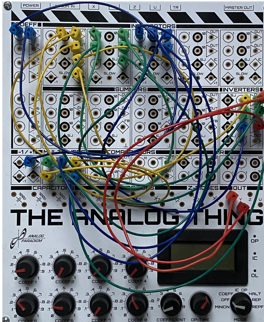
Figure 3: Setup of THE ANALOG THING for the chaotic SPROTT system
