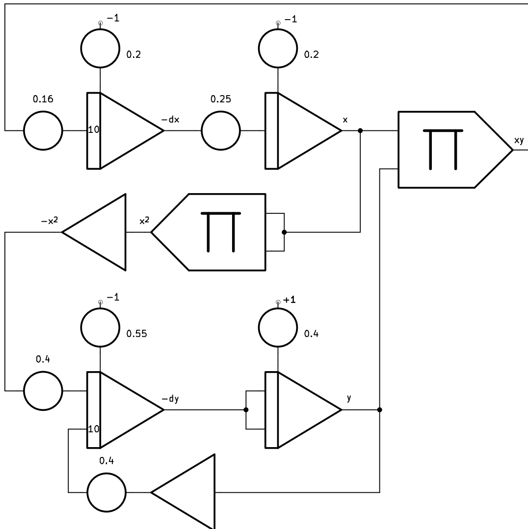
Figure 1: Program for the minimal chaotic Hamiltonian
