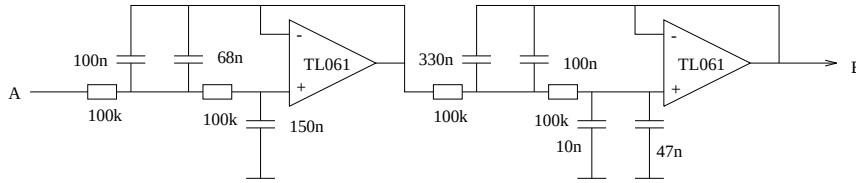
Figure 5: The four pole low pass butterworth filter
